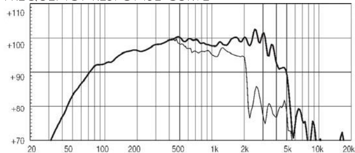
FREQUENCY RESPONSE CURVE OF 12ND830 MADE ON 50 LIT. ENCLOSURE TUNED 60HZ IN FREE FIELD (4#) ENVIRONMENT. ENCLOSURE CLOSES THE REAR OF THE DRIVER. THE THIN LINE REPRESENTS 45 DEG. OFF AXIS FREQUENCY RESPONSE.
